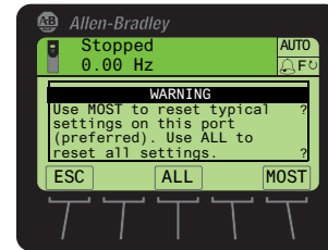
Figure 10 - 'This Port Only' Popup Box
